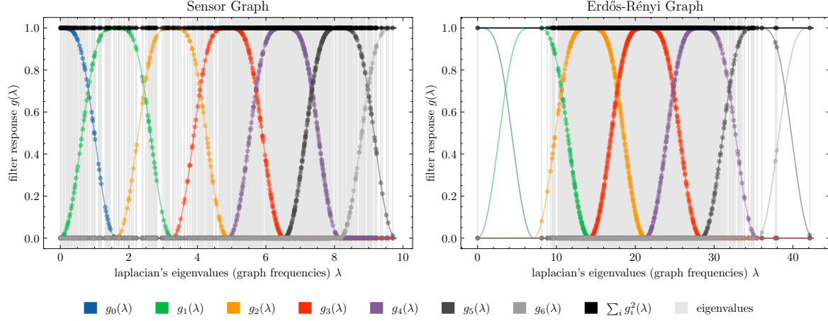
Figure 3: Itersine plot.
