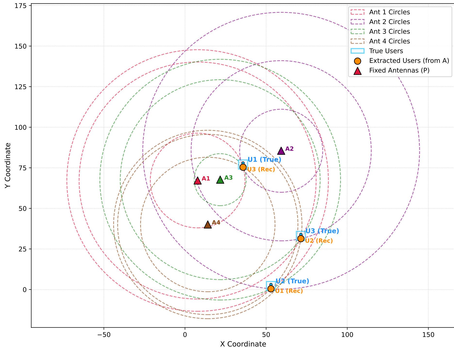
Antenna & User Scatter Plot with Distance Circles (R=3, I=4)
