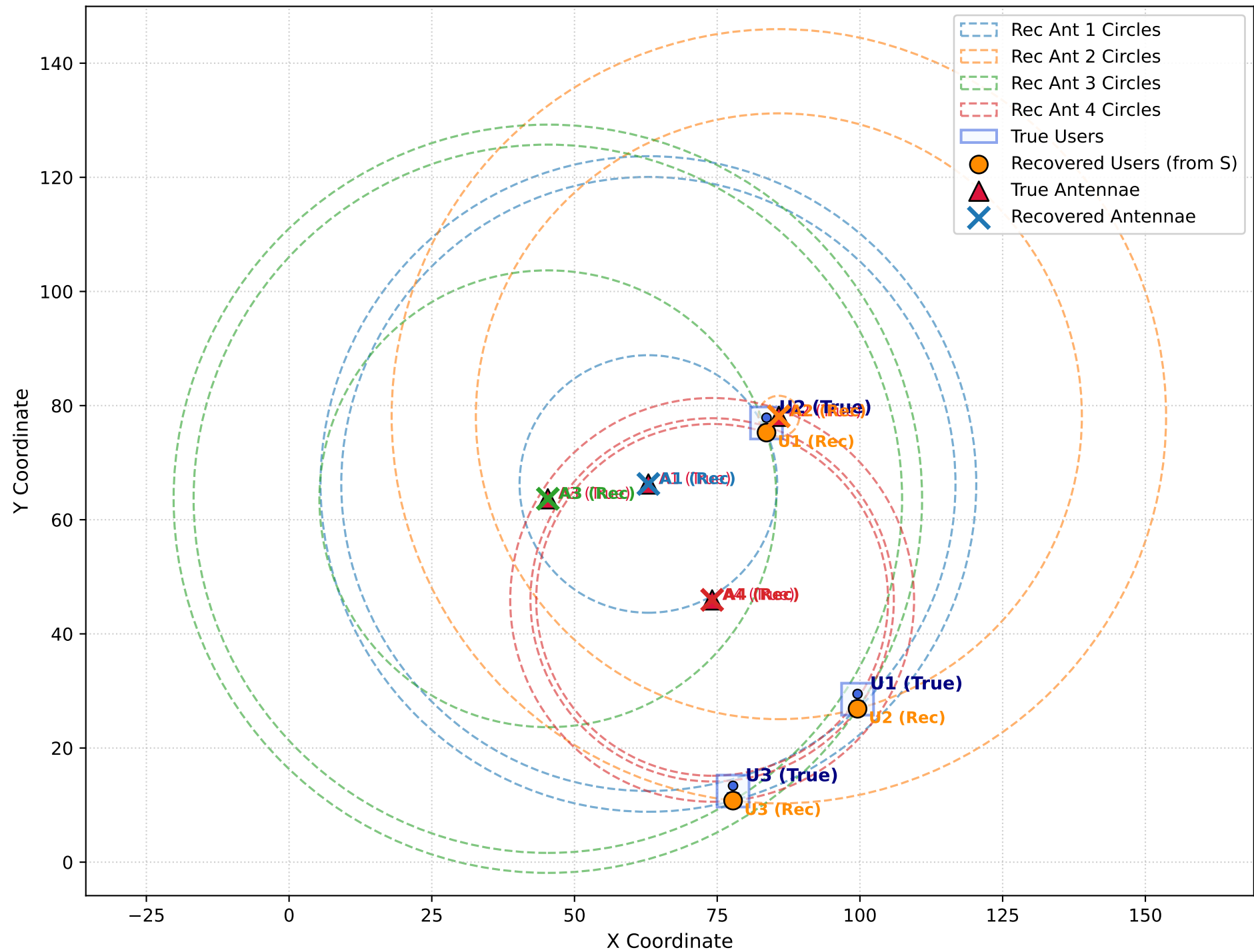
Antenna & User Scatter Plot with Distance Circles (R=3, l=4)
