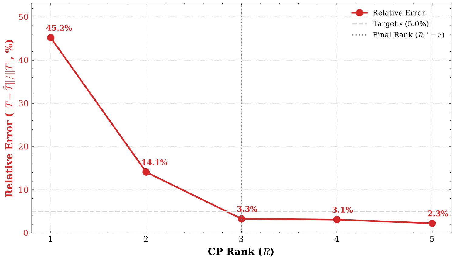
EEM CP Decomposition: Error vs Rank (Final R^* = 3 , \epsilon^* = 3.31\% )
