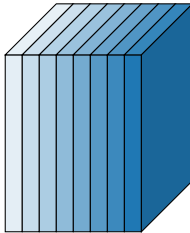
Lateral slices, T_{:,j,:} .
