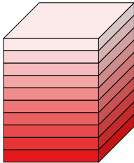
Horizontal slices, T_{i,:,:} .
