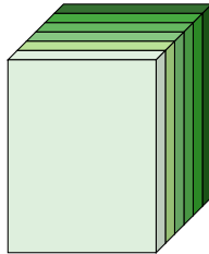
Frontal slices, T_{:,:,k} .
