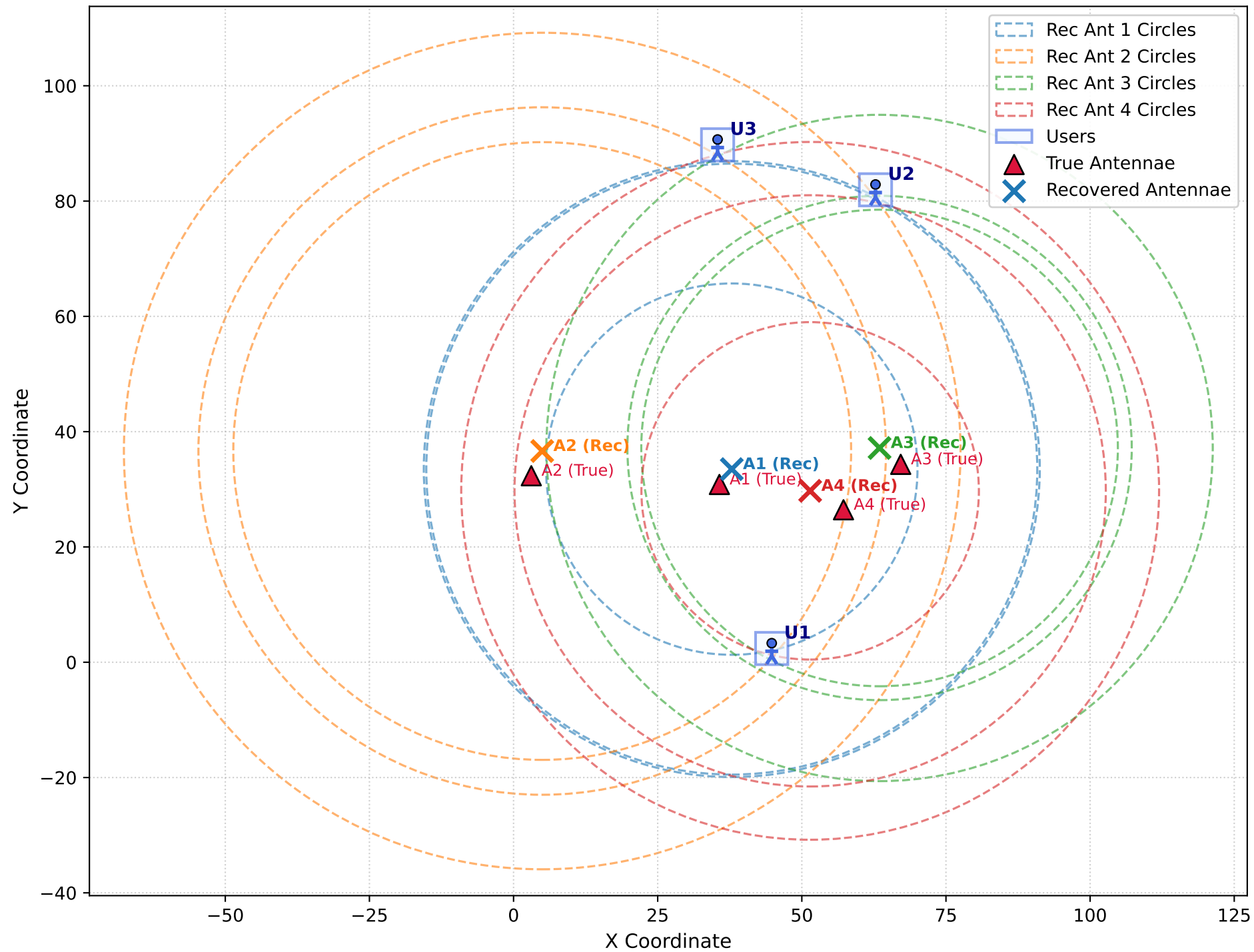
DS-CDMA Antenna & User Scatter Plot with Distance Circles ( R=3 , l=4 )
