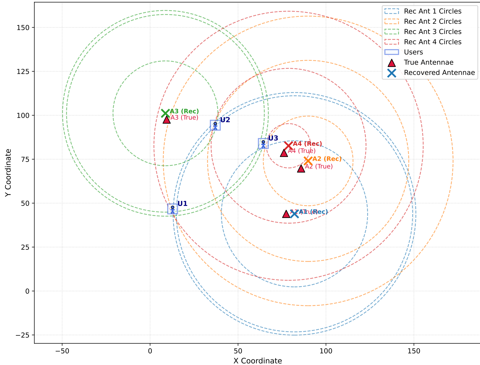
DS-CDMA Antenna & User Scatter Plot with Distance Circles (R=3, l=4)
