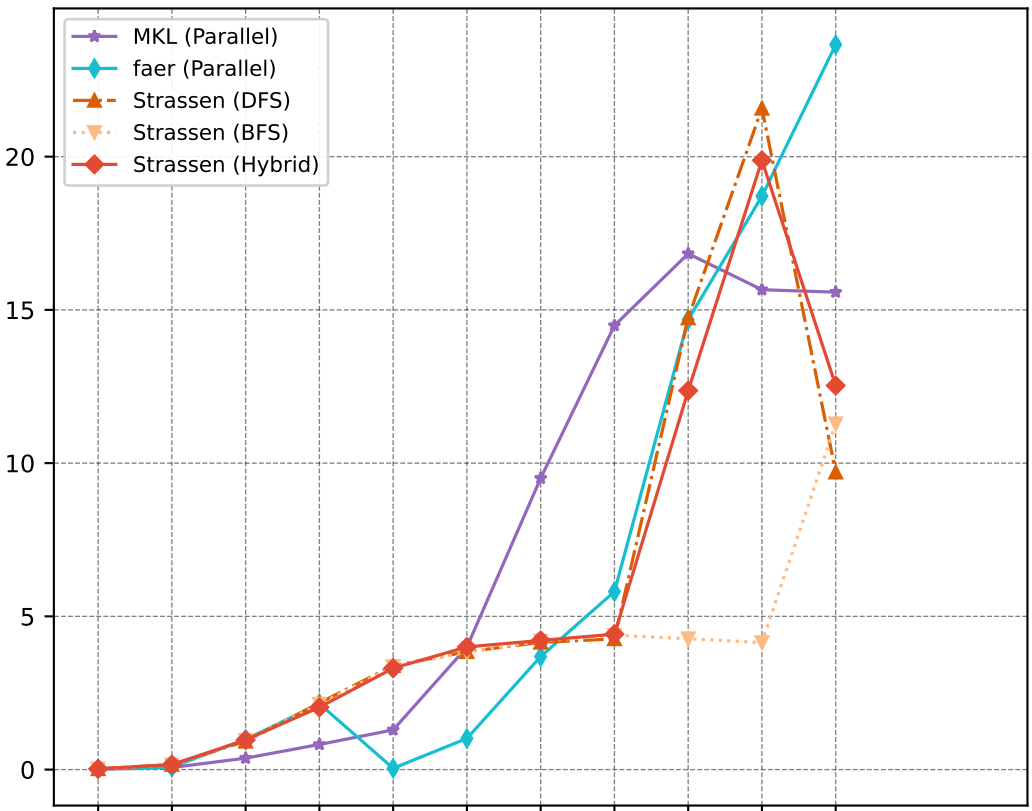
Parallel Algorithms
