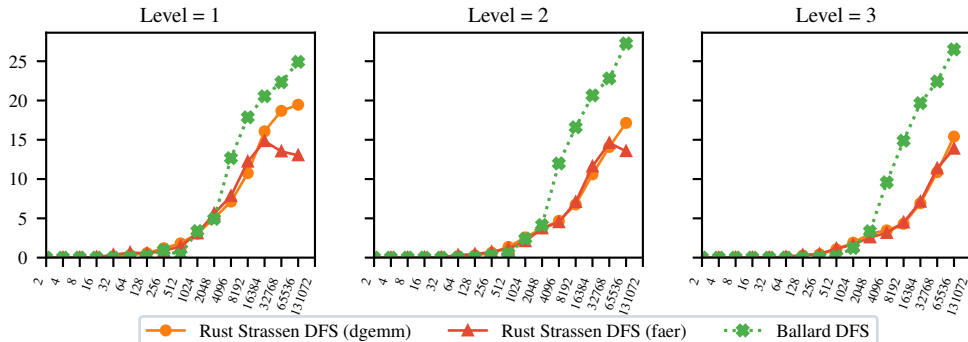
[DFS] Effective GFLOPS / core
