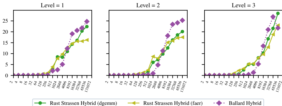
[HYBRID] Effective GFLOPS / core
