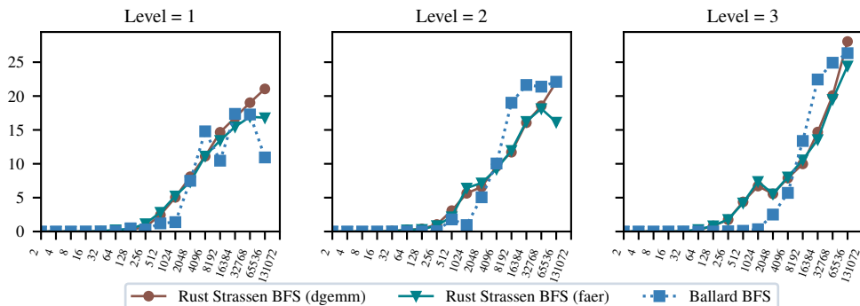
[BFS] Effective GFLOPS / core
