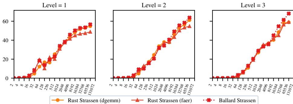
[SEQ] Effective GFLOPS
