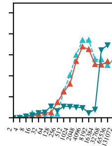
Cutoff = 16384
