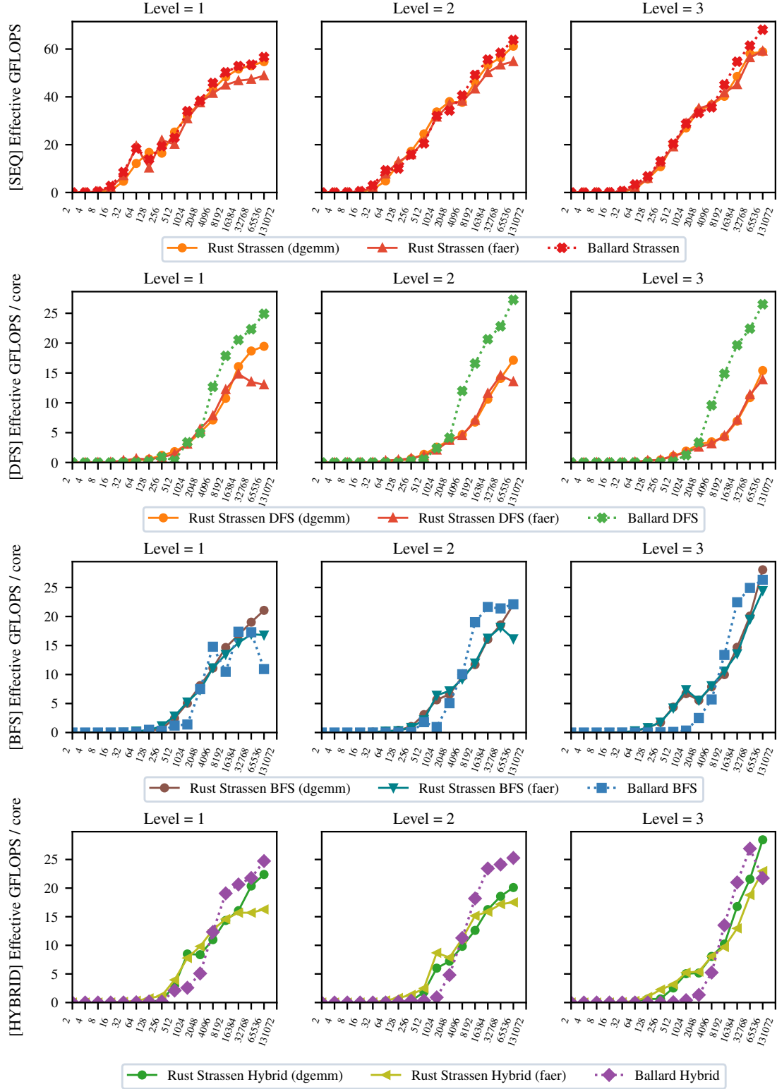
Figure 9: Performance comparison of our Rust Strassen implementation (using dgemm and faer base cases) against the Benson & Ballard reference benchmarks across sequential and parallel execution modes.
