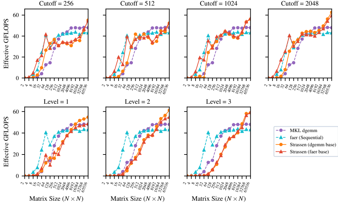
Sequential Matrix Multiplication Performance Comparison
