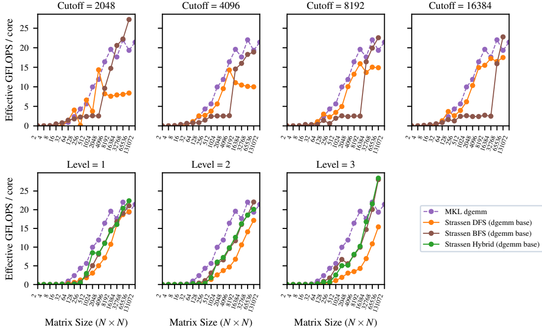
Figure 5: Parallel matrix multiplication performance comparison (normalized per core) of Strassen variants (DFS, BFS, Hybrid) against parallel dgemm across cutoff sizes (2048, 4096, 8192, 16384) in the first row, and recursion levels (1, 2, 3) in the second row.
