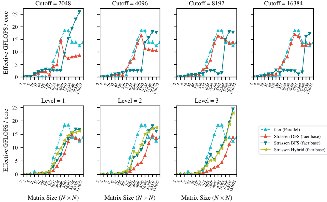
Figure 6: Parallel matrix multiplication performance comparison (normalized per core) of Strassen variants (DFS, BFS, Hybrid) against parallel faer across cutoff sizes (2048, 4096, 8192, 16384) in the first row, and recursion levels (1, 2, 3) in the second row.
