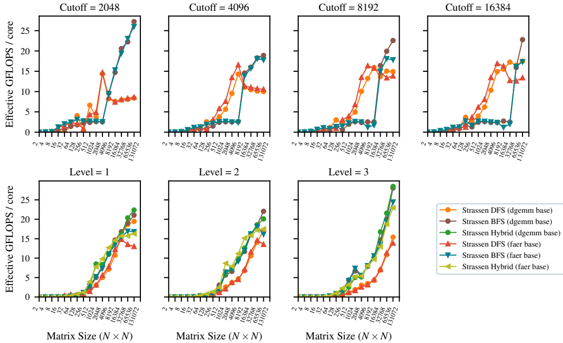
Figure 4: Parallel matrix multiplication performance comparison (normalized per core) of Strassen variants (DFS, BFS, Hybrid) across cutoff sizes (2048, 4096, 8192, 16384) in the first row, and recursion levels (1, 2, 3) in the second row.
