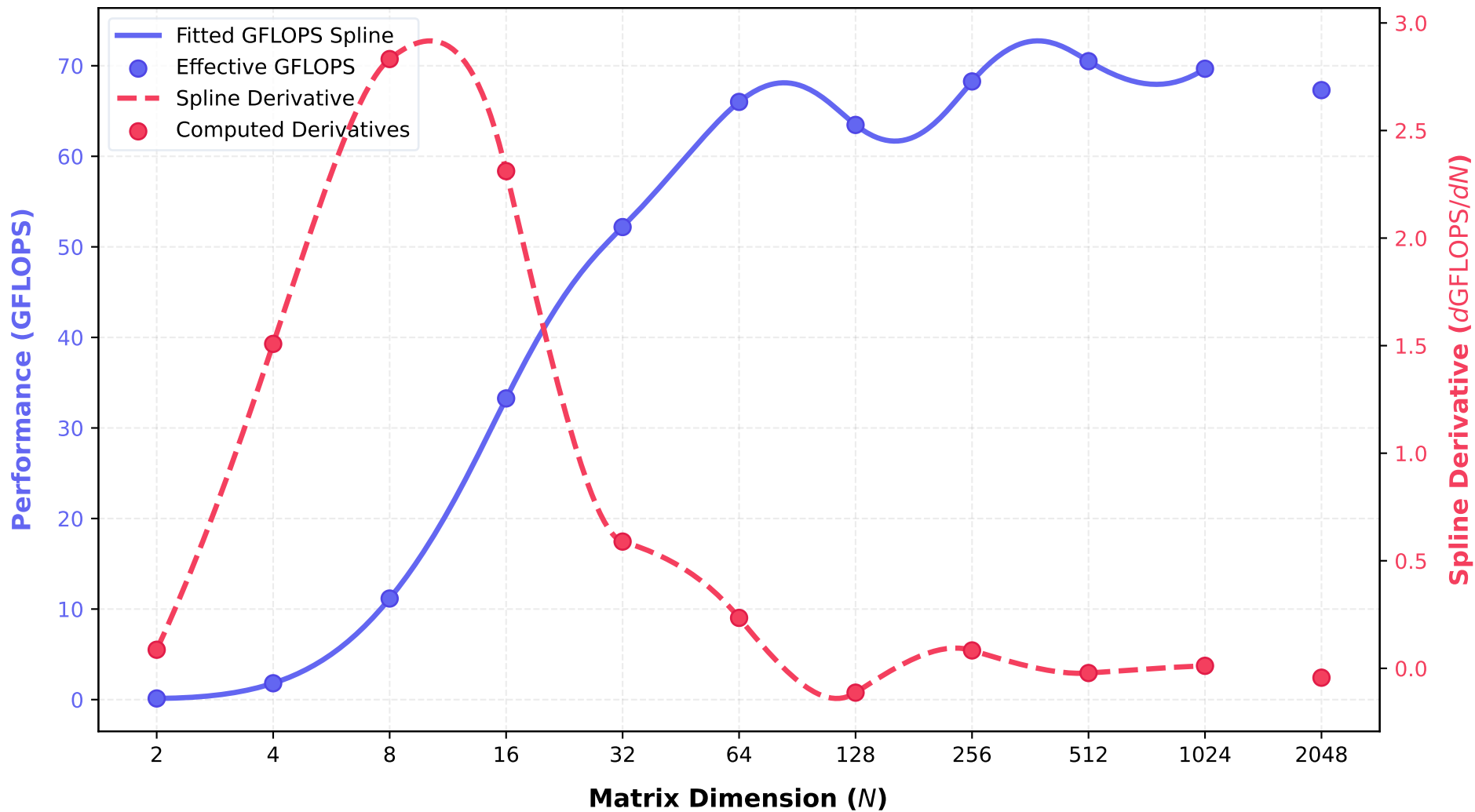
Baseline Matrix Multiplication GFLOPS Performance & Spline Derivative
