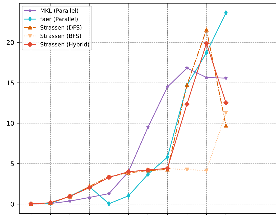
Parallel Algorithms
