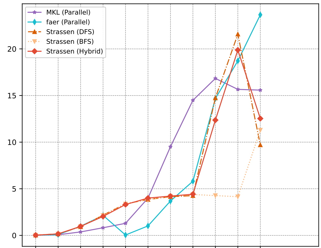
Parallel Algorithms
