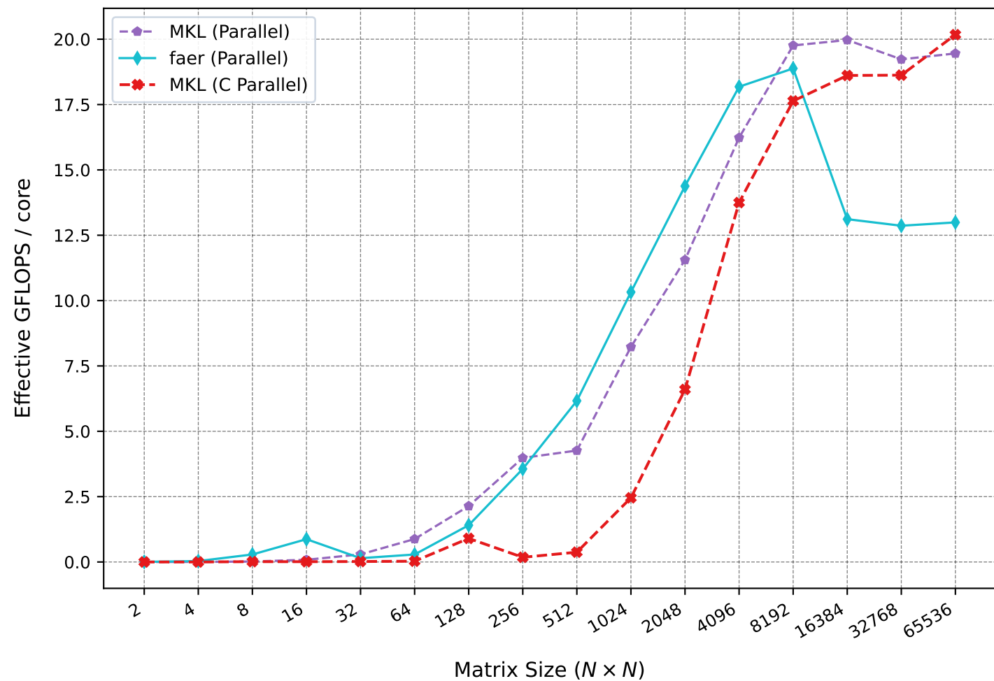
Parallel Execution (Normalized per Core)
