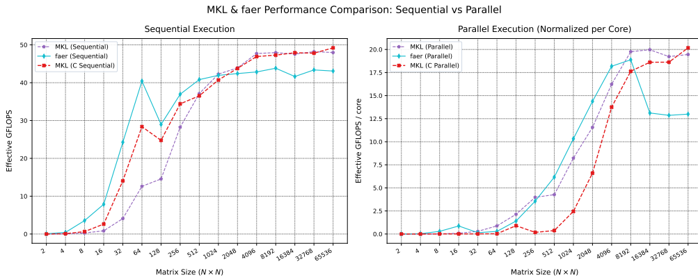
Figure 2: Comparison between MKL and faer in sequential and parallel execution.
