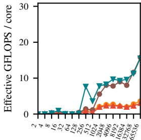
Cutoff = 4096
