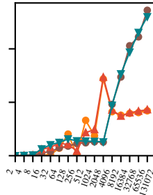
Cutoff = 2048
