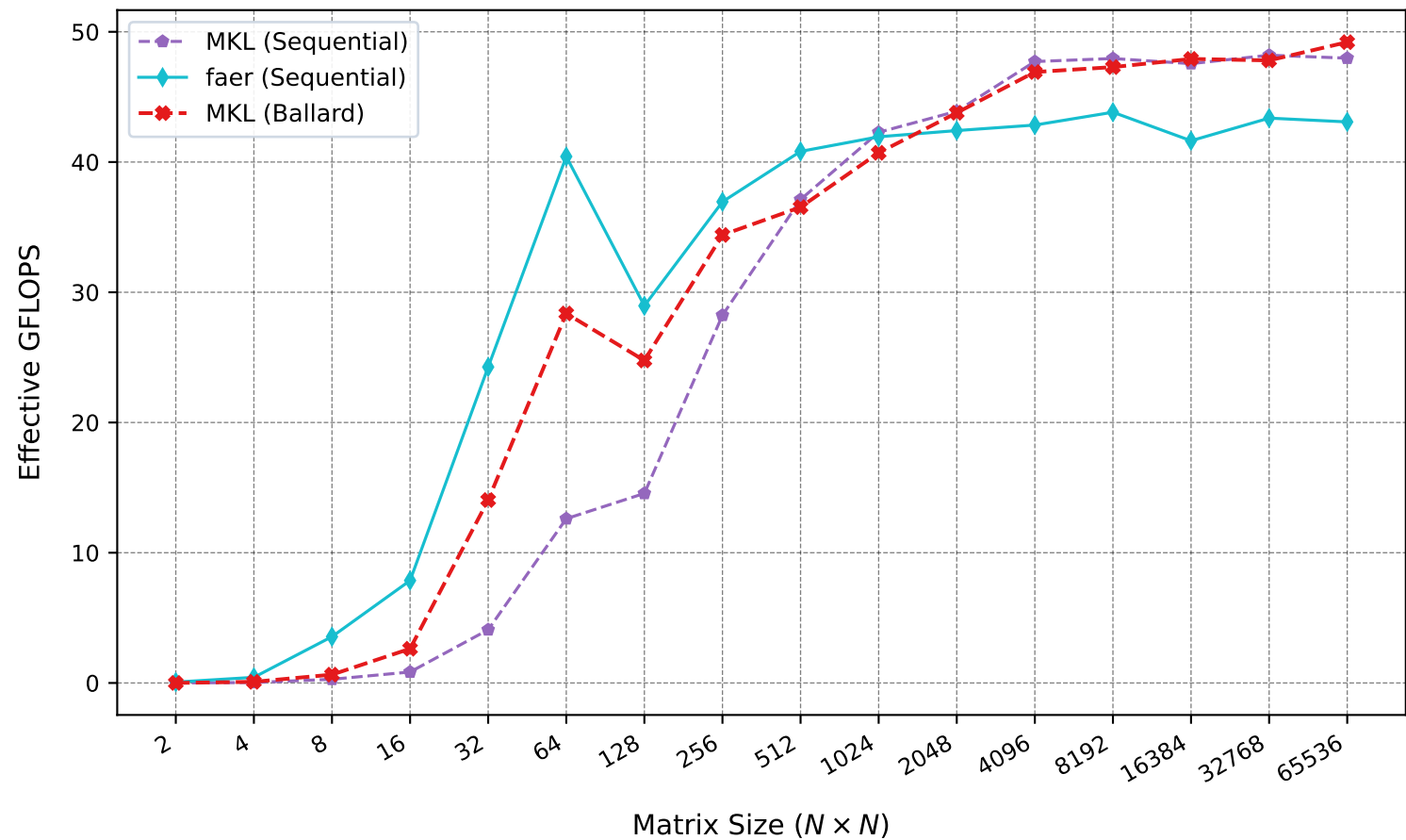
Sequential Matrix Multiplication Performance Comparison MKL, faer, and MKL (Ballard)
