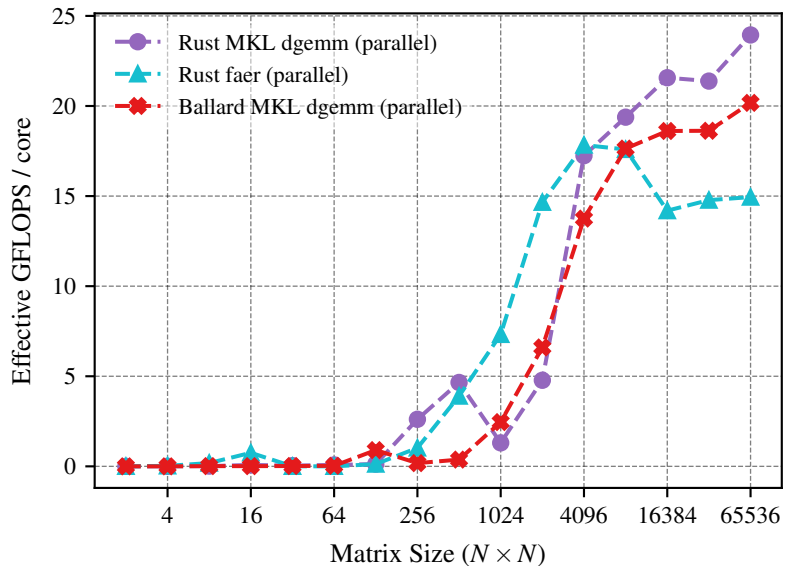
Parallel Execution (Normalized per Core)
