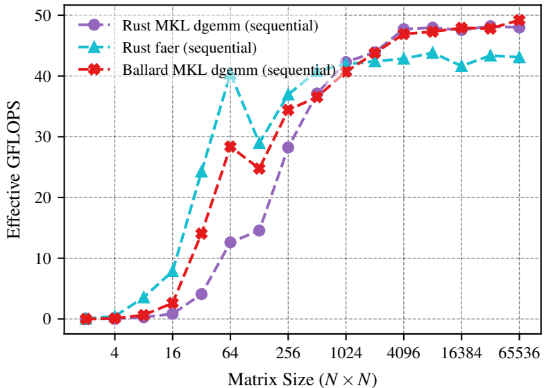
Sequential Execution
