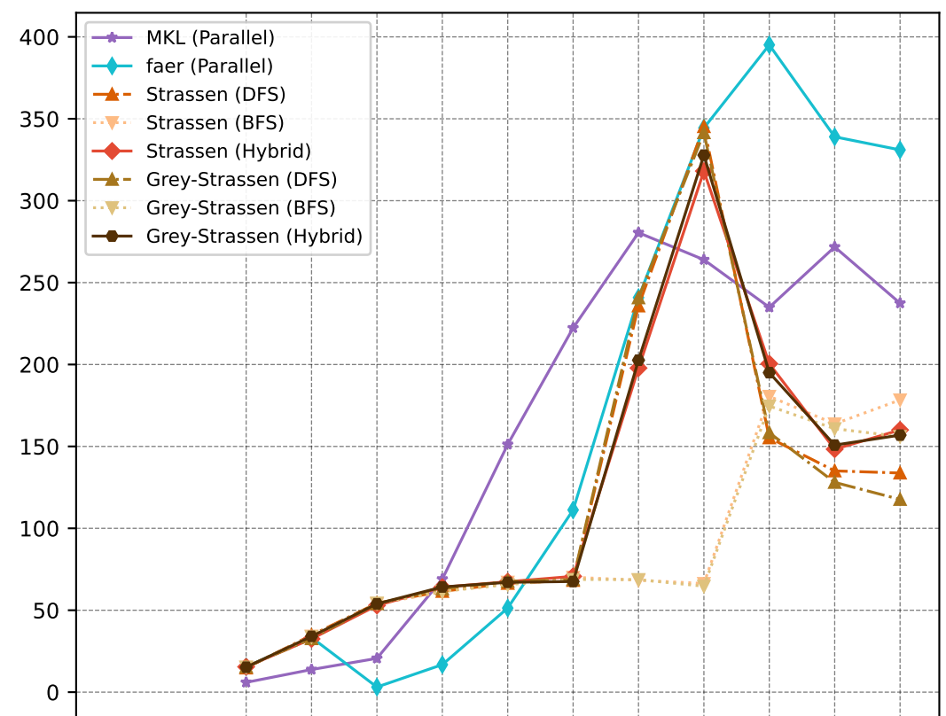
Parallel Algorithms
