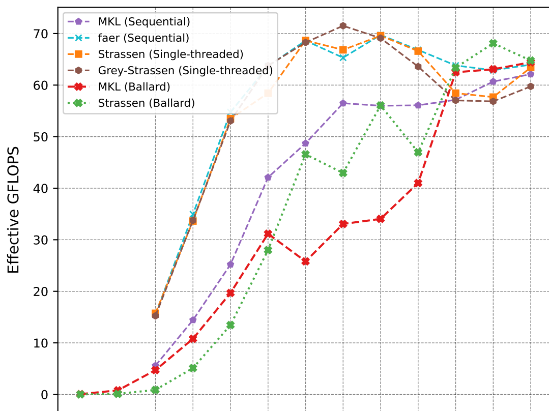
Sequential Algorithms
