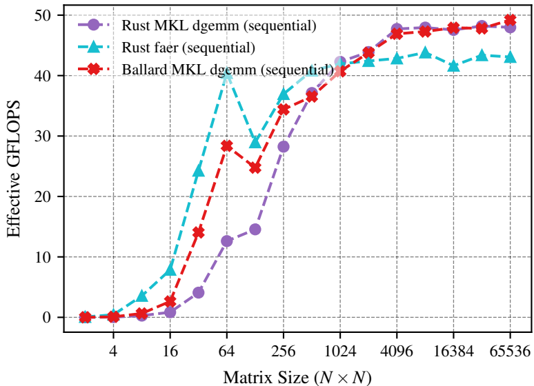
Sequential Execution
