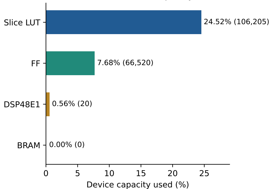
A Resource occupancy
