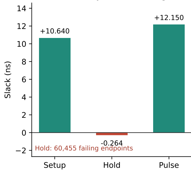
B Post-synthesis timing
