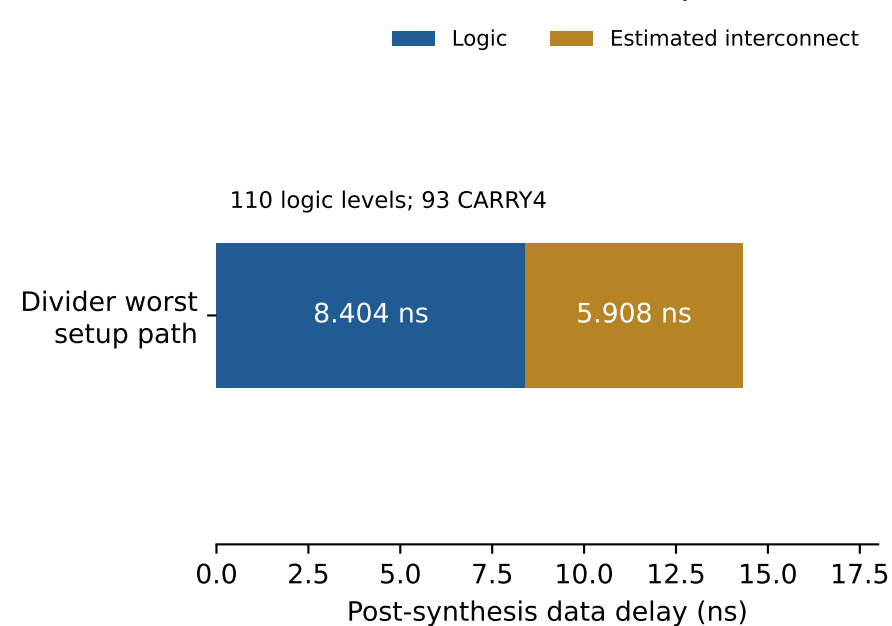
C Critical arithmetic path
