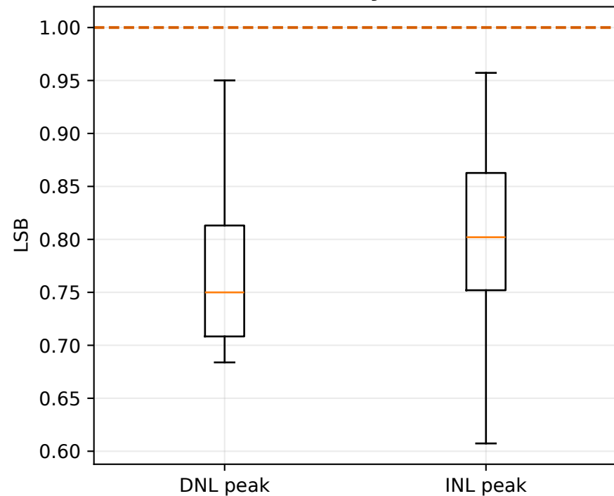
Exact code-density static metrics
