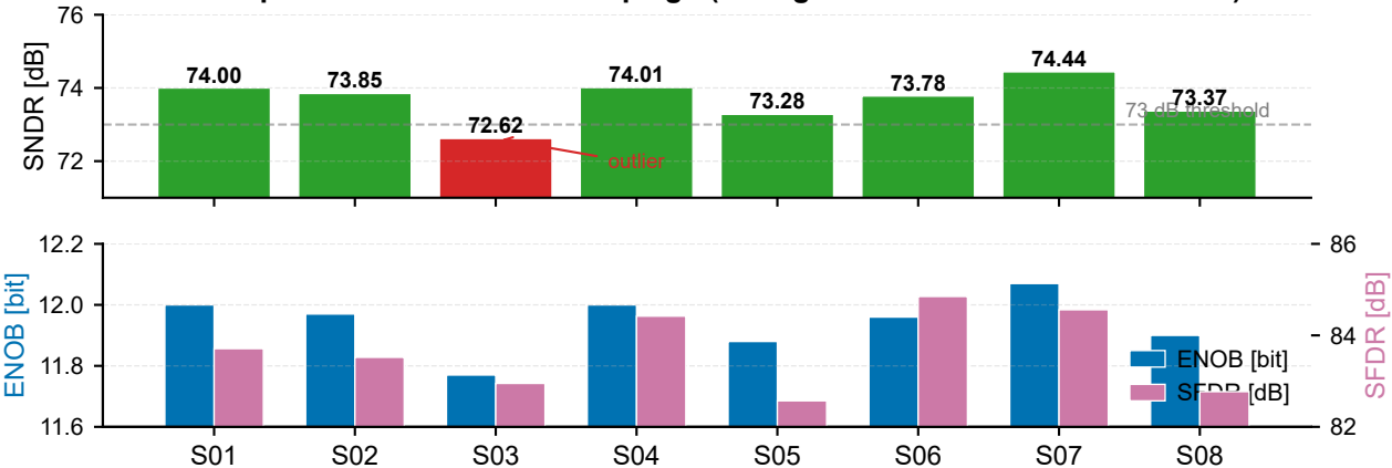
8-Sample Omran Mismatch Campaign (Huang Calibration + 1LSB Deadband)
