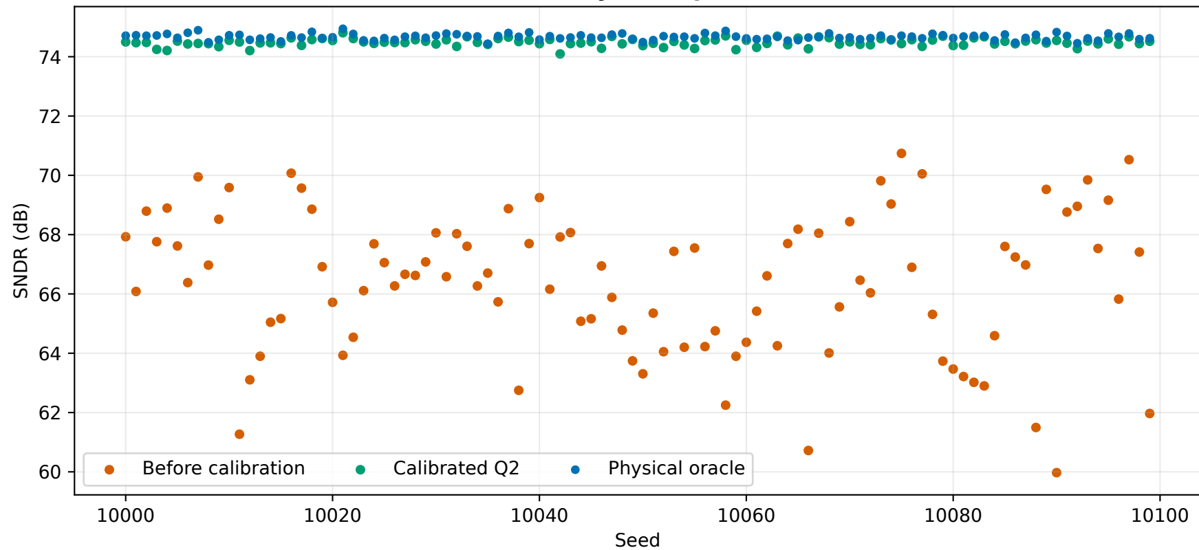
Monte Carlo dynamic performance
