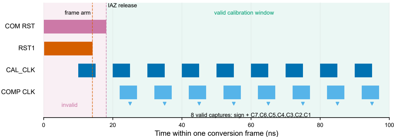
(b) Frame-synchronous comparator usage
