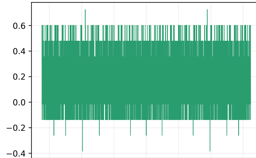
Calibration + SRM
