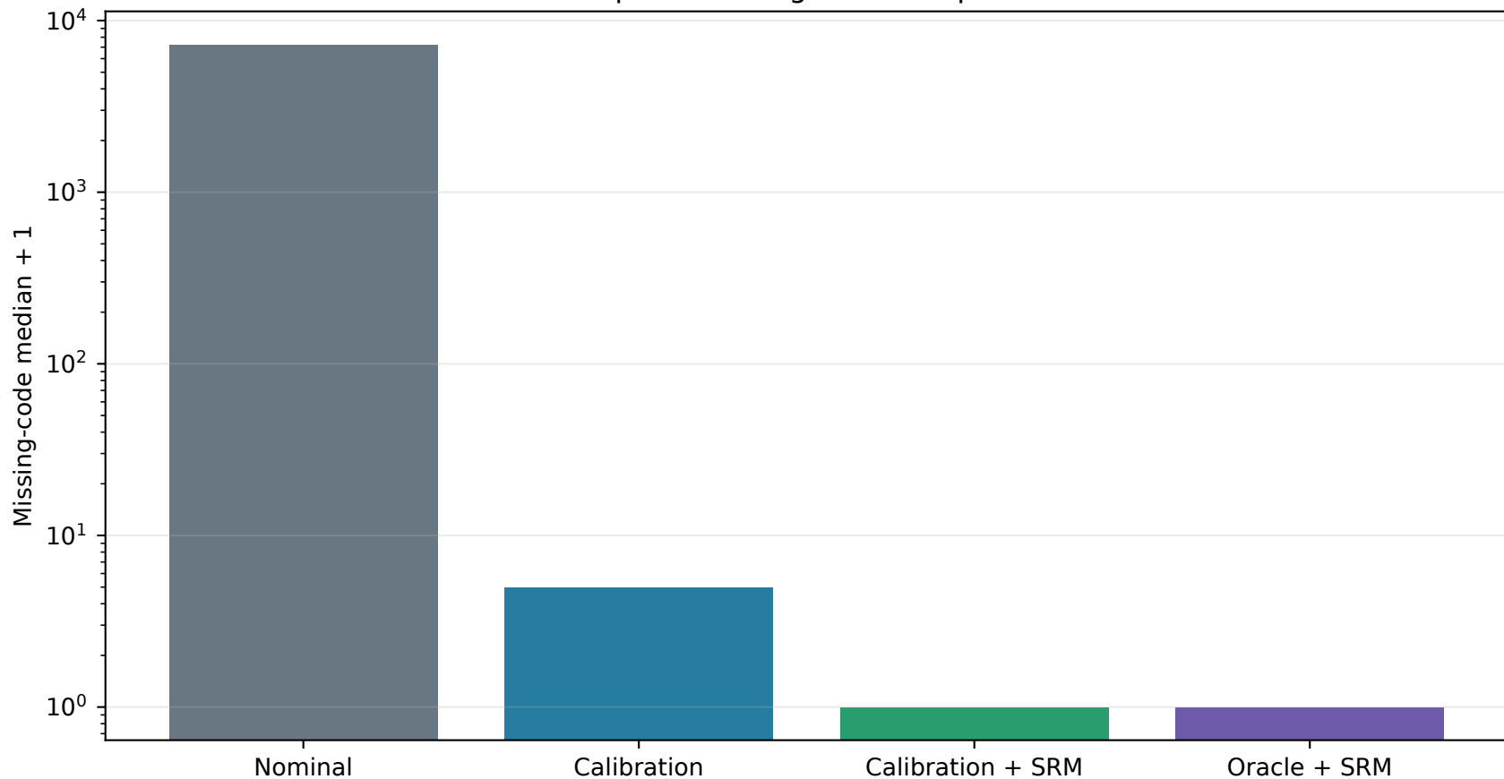
512-point missing-code comparison
