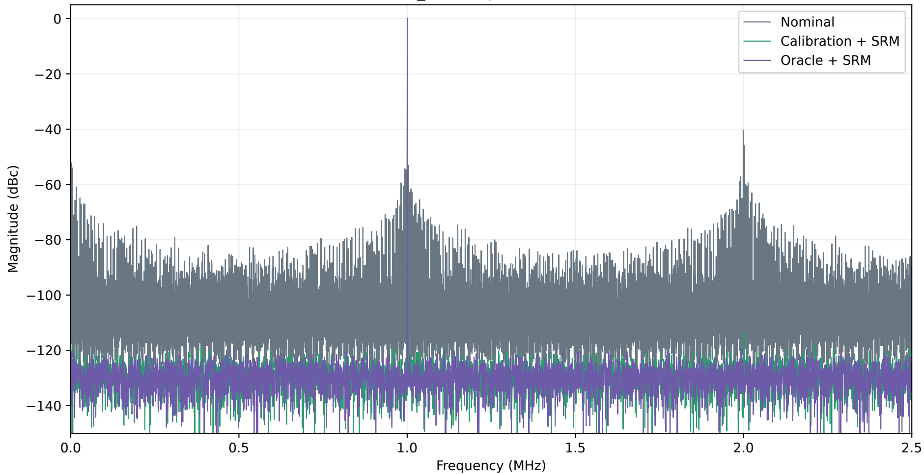
Best CAL_SRM chip 50: coherent FFT
