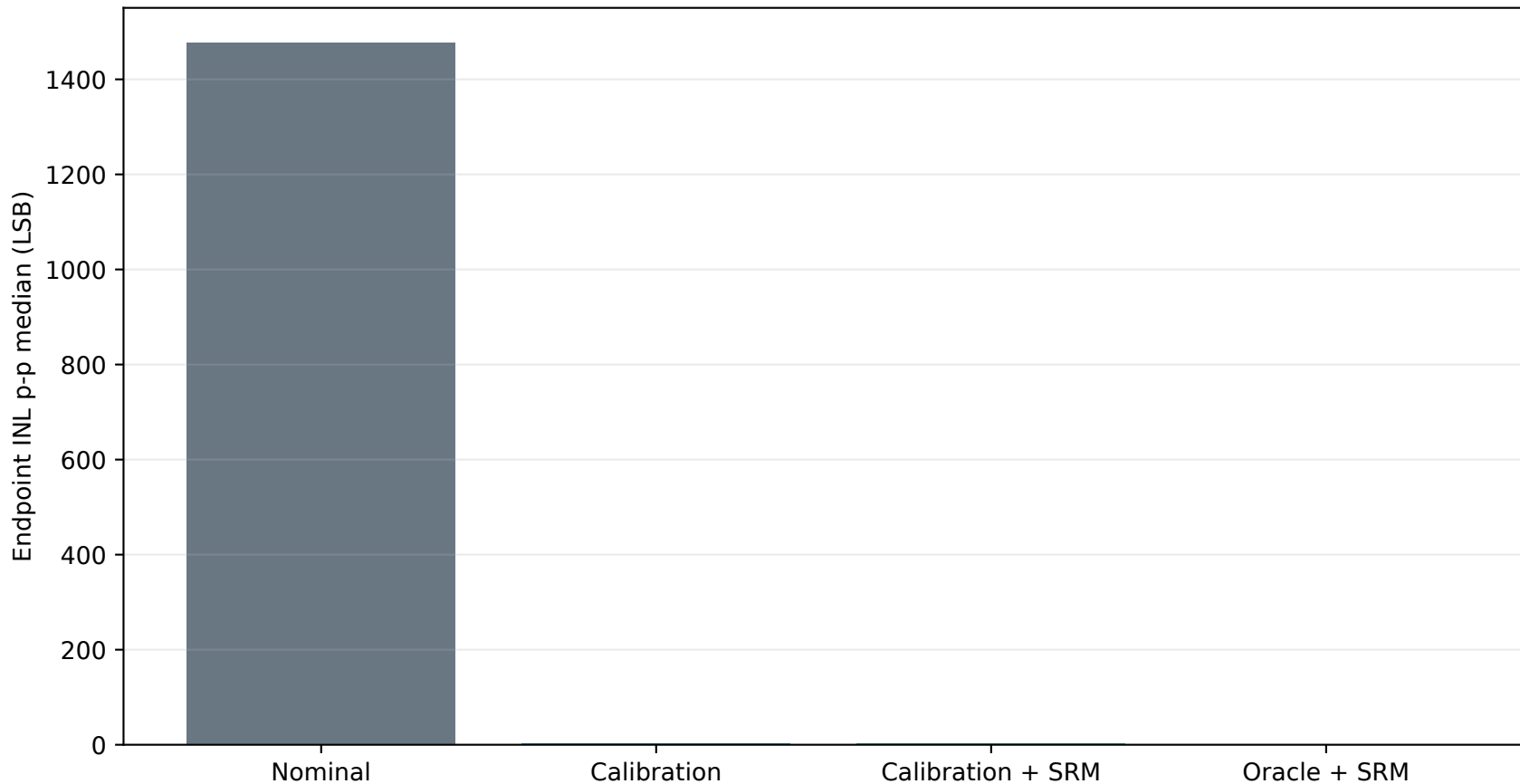
512-point full-range ramp linearity
