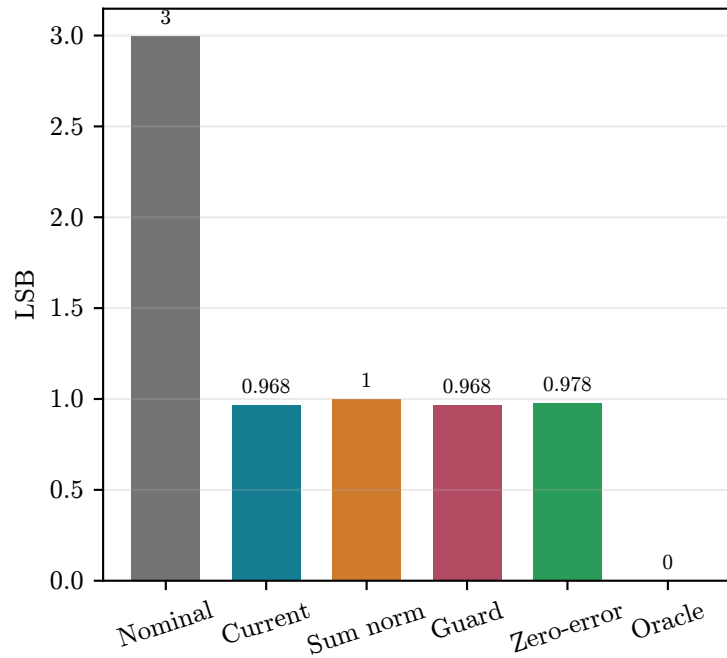
DNL max median
