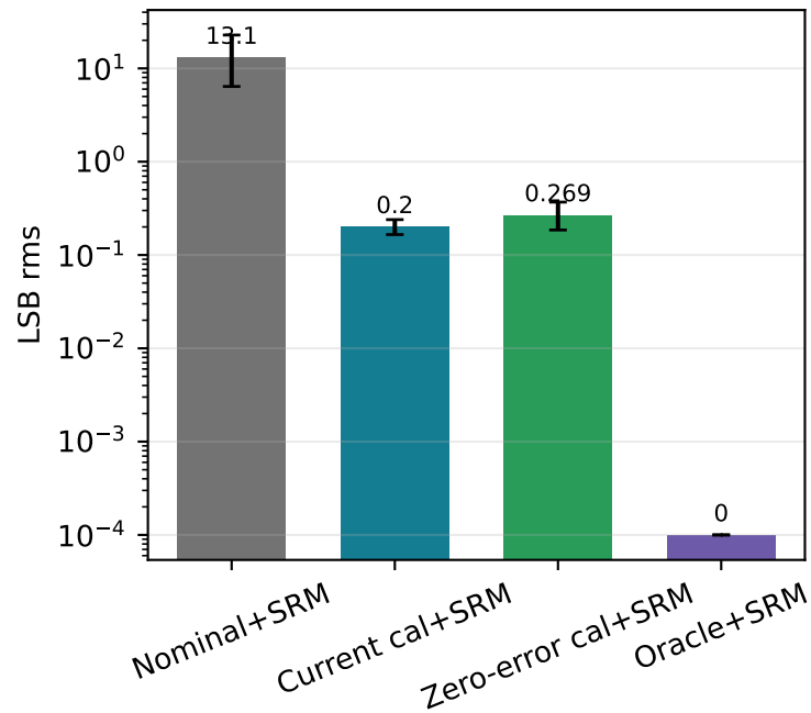
Weight error
