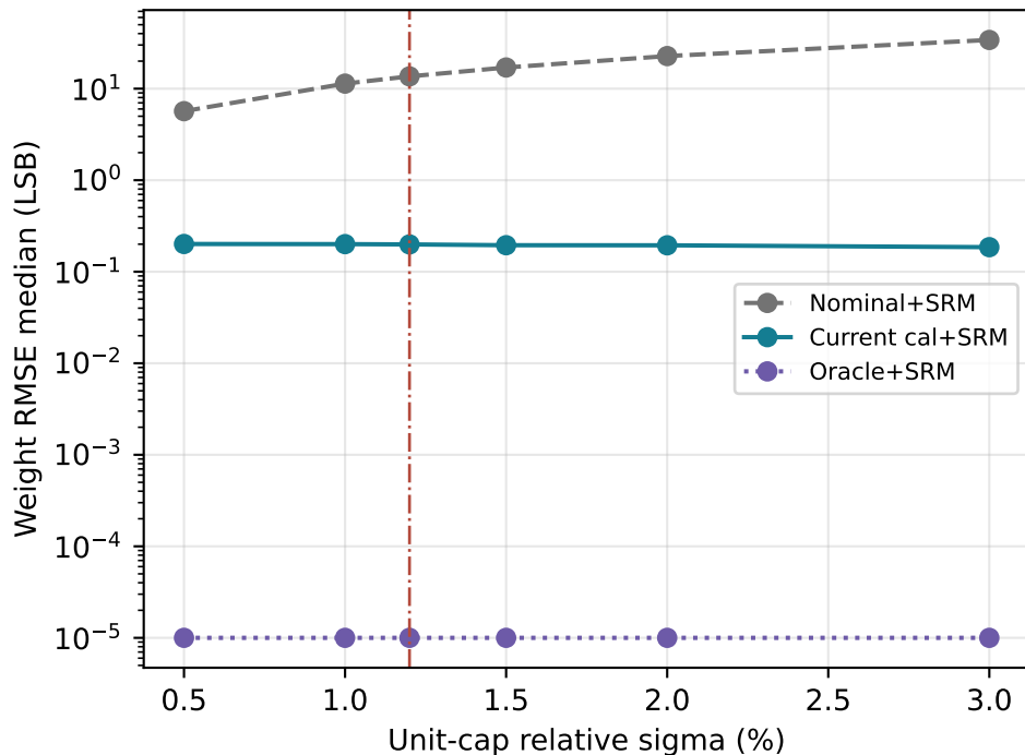
Physical unit-cap mismatch sensitivity, 128 chips per point
