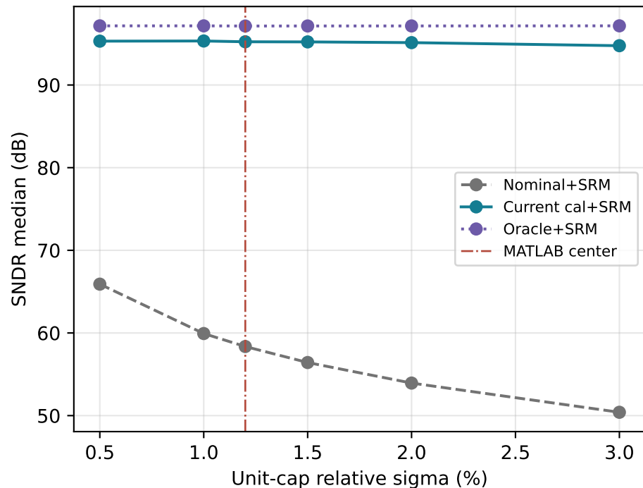
Physical unit-cap mismatch sensitivity, 128 chips per point
