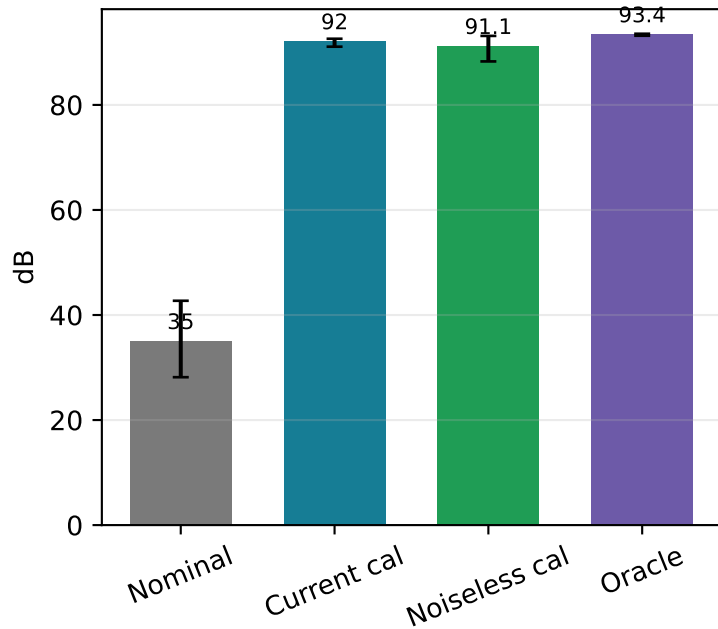
Noiseless dynamic SNDR
