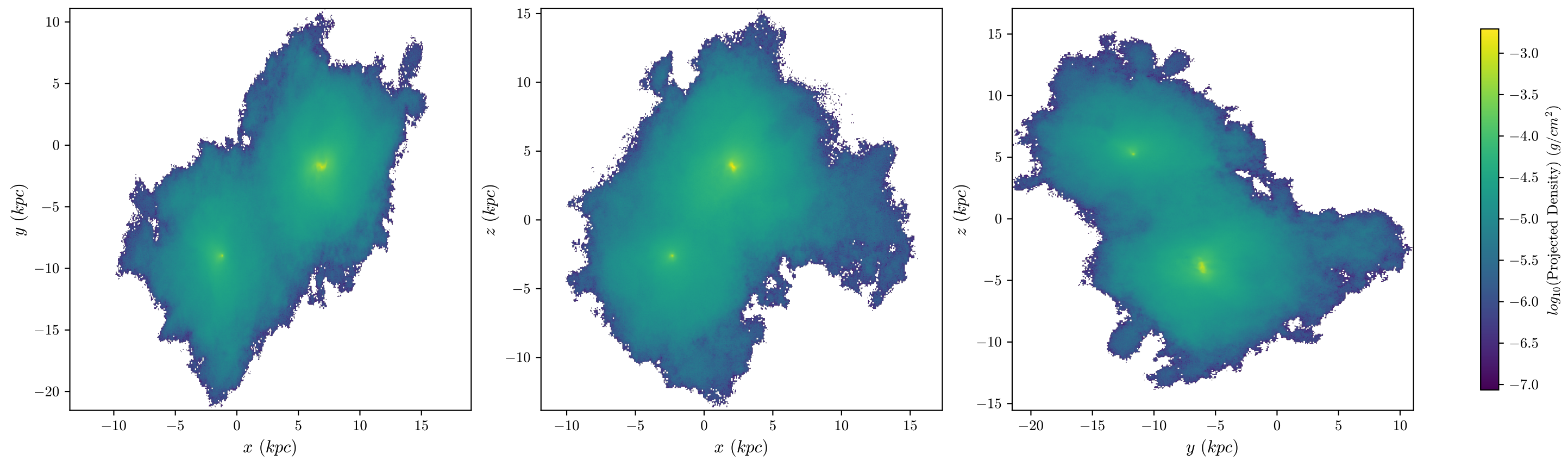
T1 Aug Neutral Hydrogen Fraction, z = 2.494 , 512 bins
