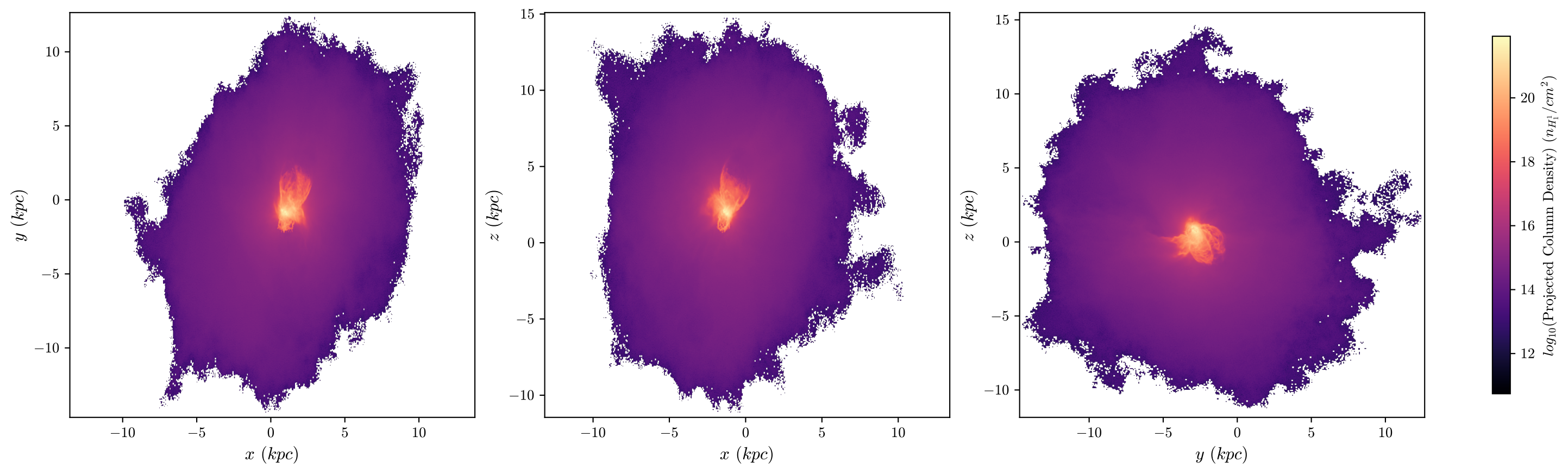
T1 Aug Neutral Hydrogen Fraction, z = 2.208 , 512 bins
