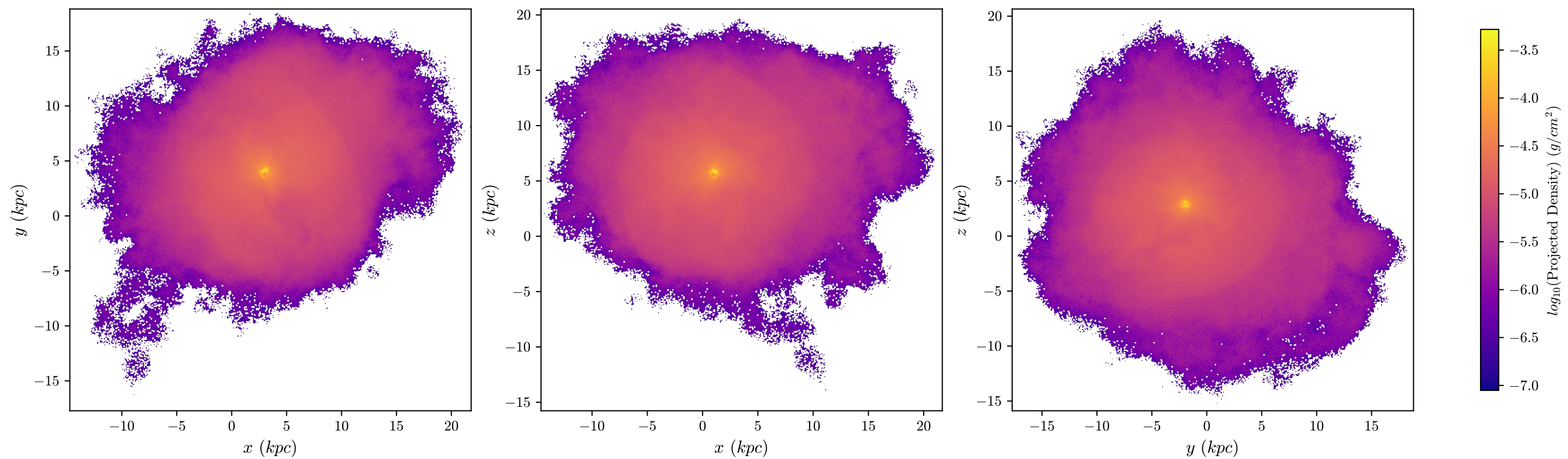
T1 Aug Hydrogen Mass Fraction, z = 1.449 , 512 bins
