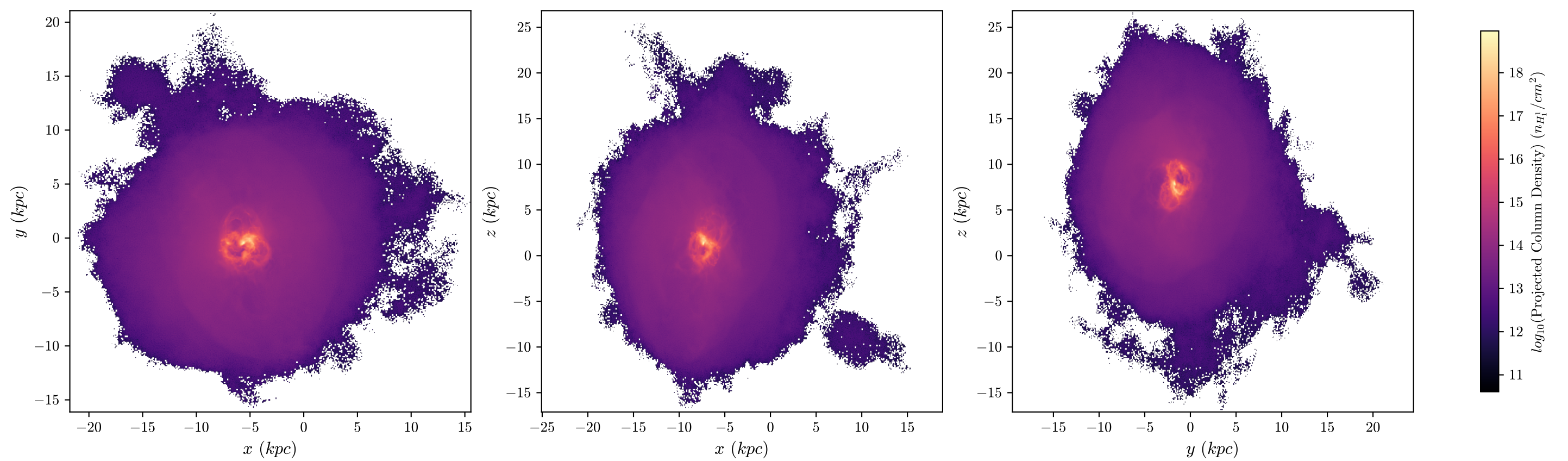
T1 Aug Neutral Hydrogen Fraction, z = 1.313 , 512 bins
