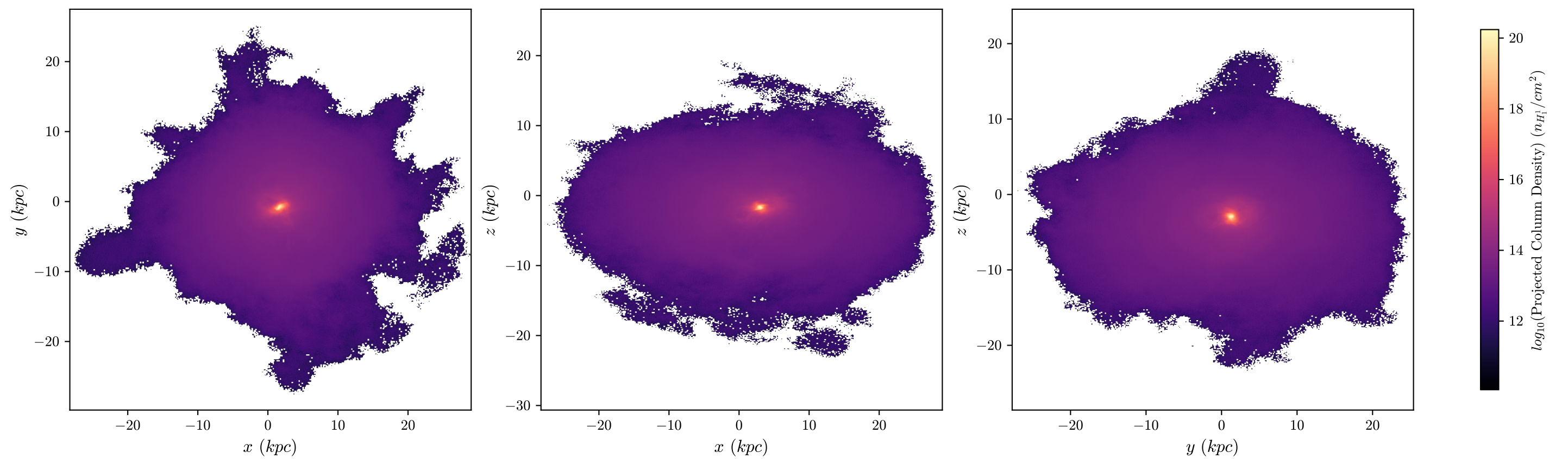
T1 Aug Neutral Hydrogen Fraction, z = 0.914 , 512 bins
