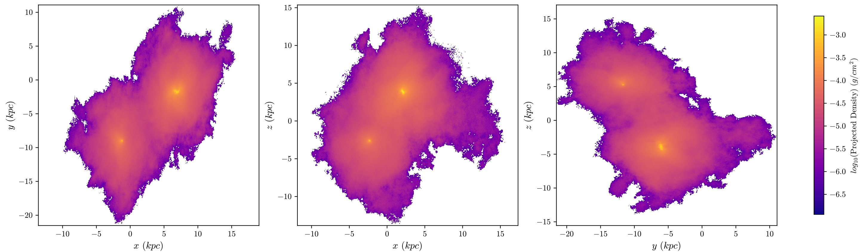
T1 Aug Dark Matter, z = 2.494 , 512 bins
