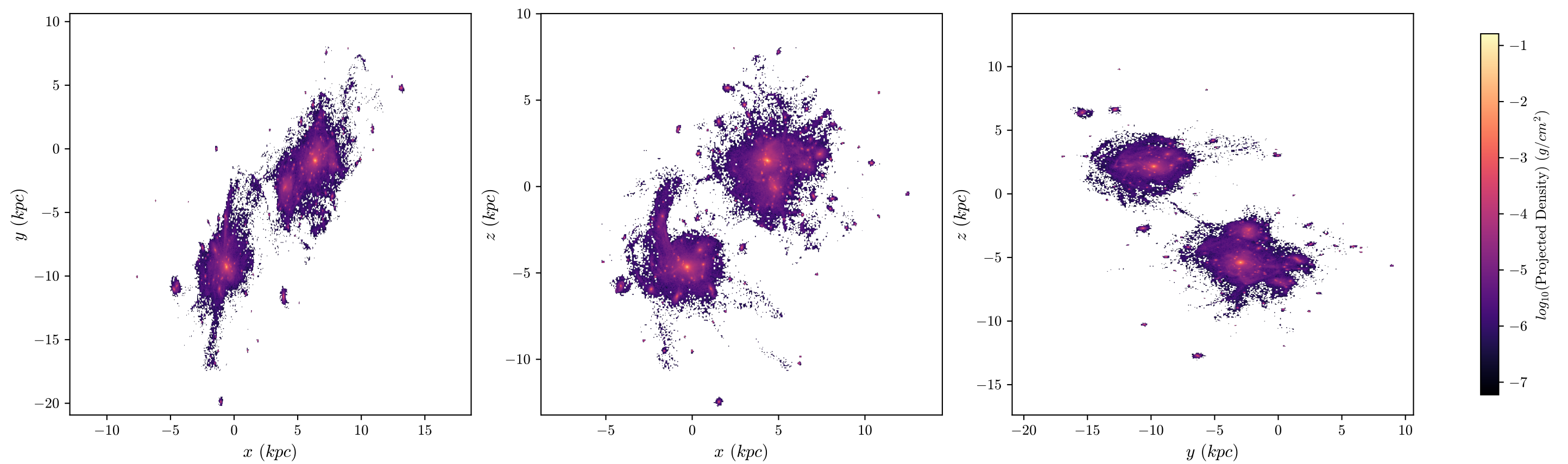
T1 Aug Stars, z = 2.494 , 512 bins
