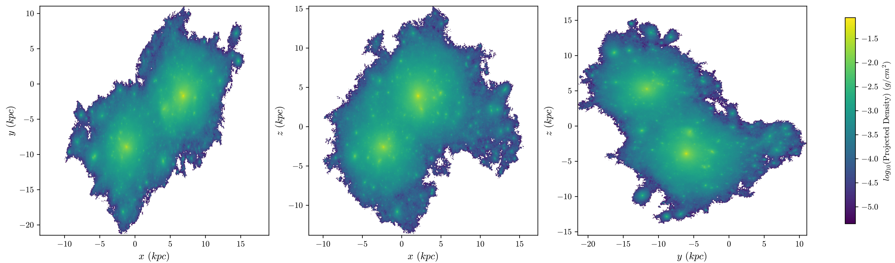
T1 Aug Stars, z = 2.494 , 512 bins
