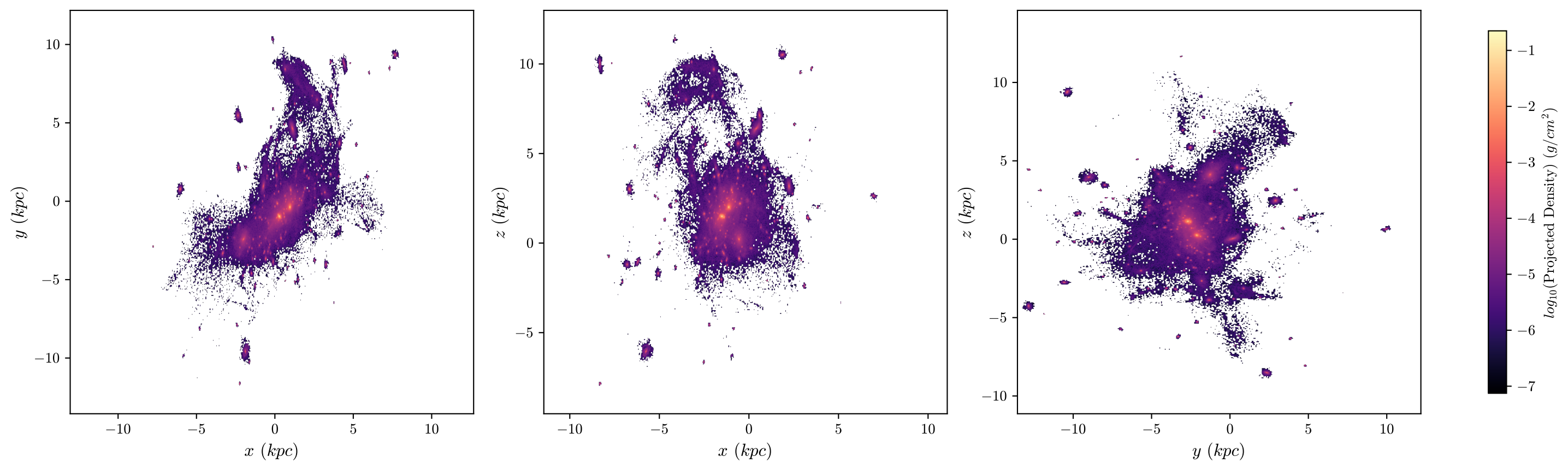
T1 Aug Stars, z = 2.208 , 512 bins
