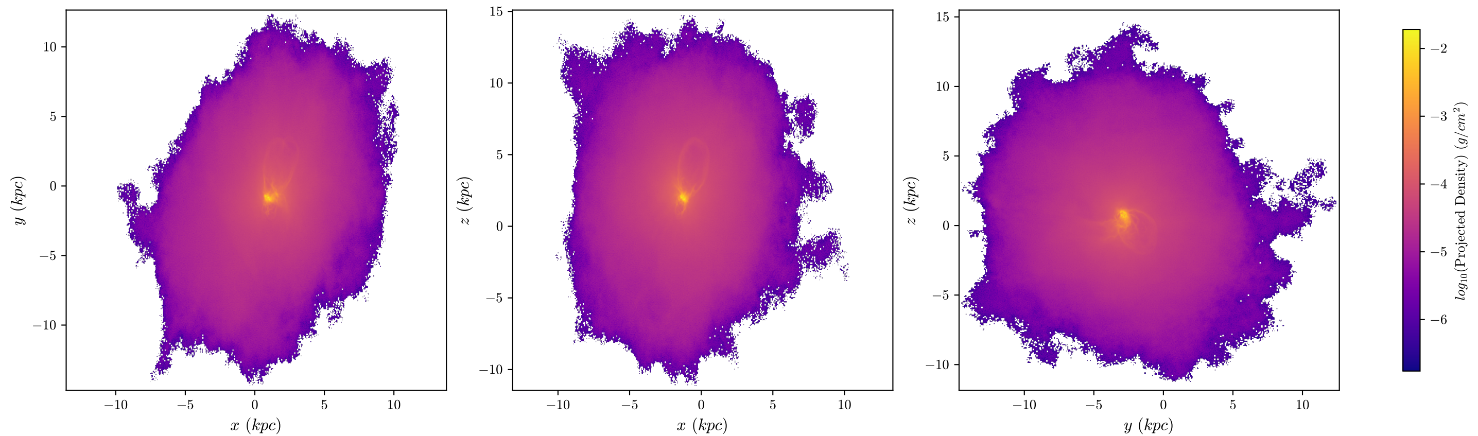
T1 Aug Dark Matter, z = 2.208 , 512 bins
