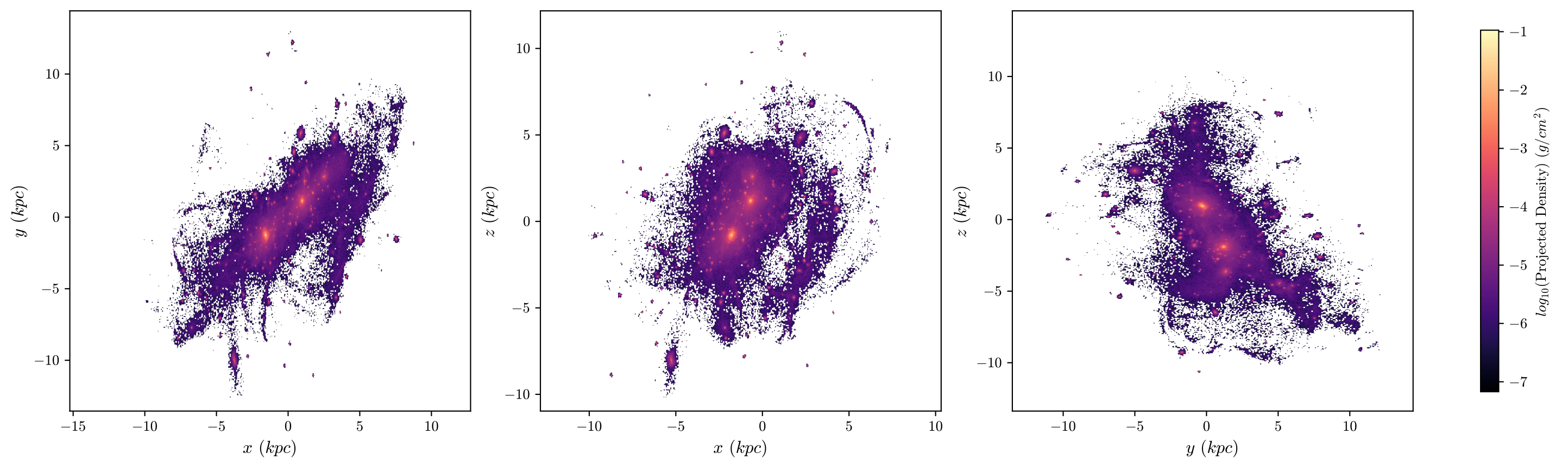
T1 Aug Stars, z = 1.96 , 512 bins
