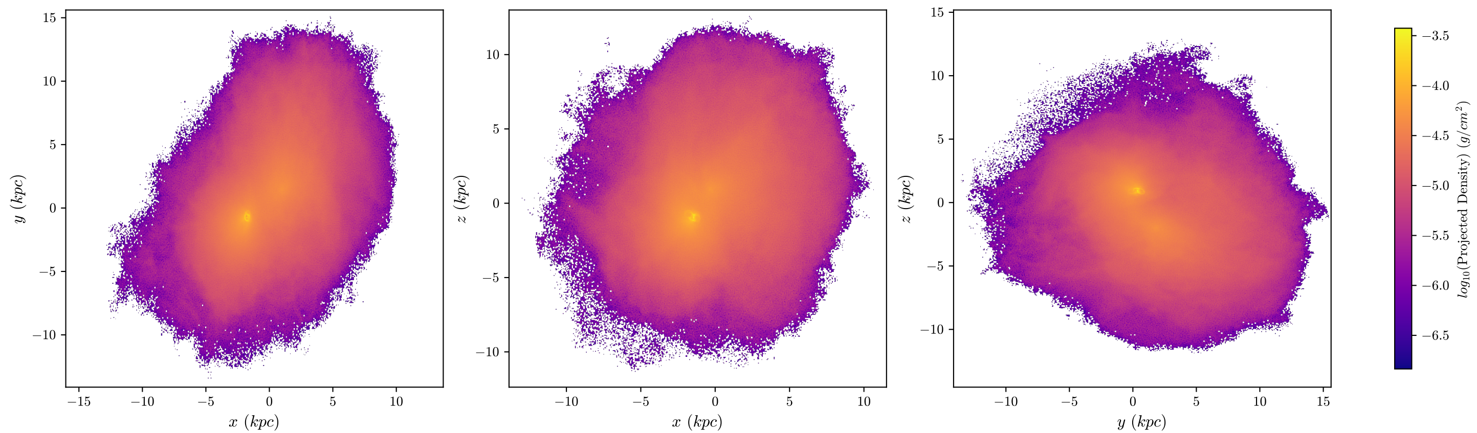
T1 Aug Dark Matter, z = 1.96 , 512 bins
