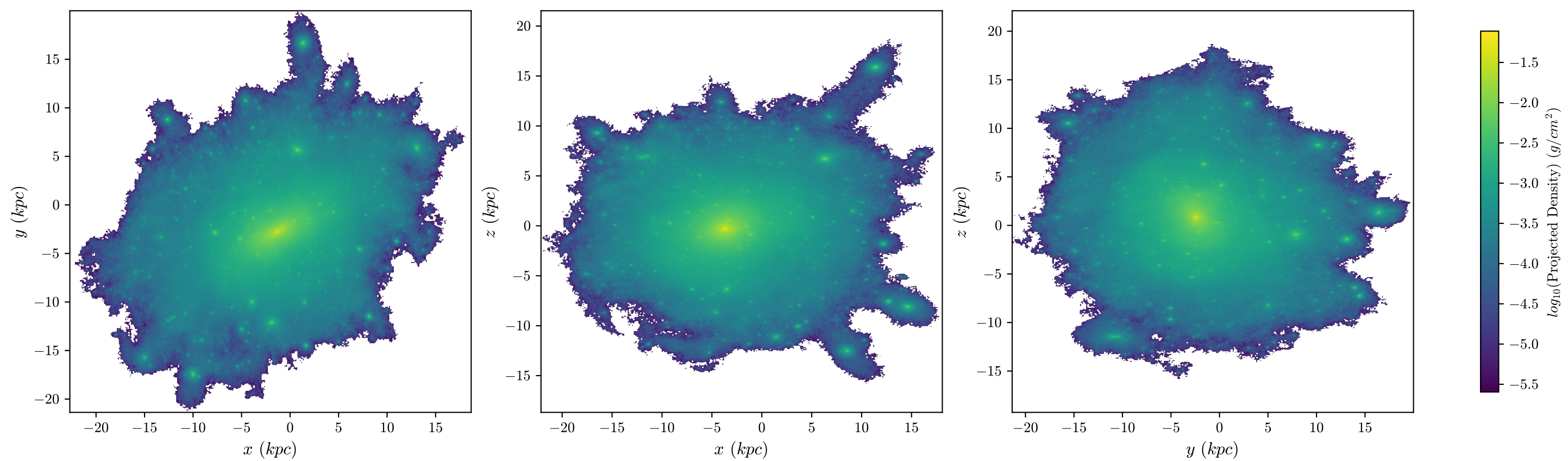
T1 Aug Stars, z = 1.592 , 512 bins
