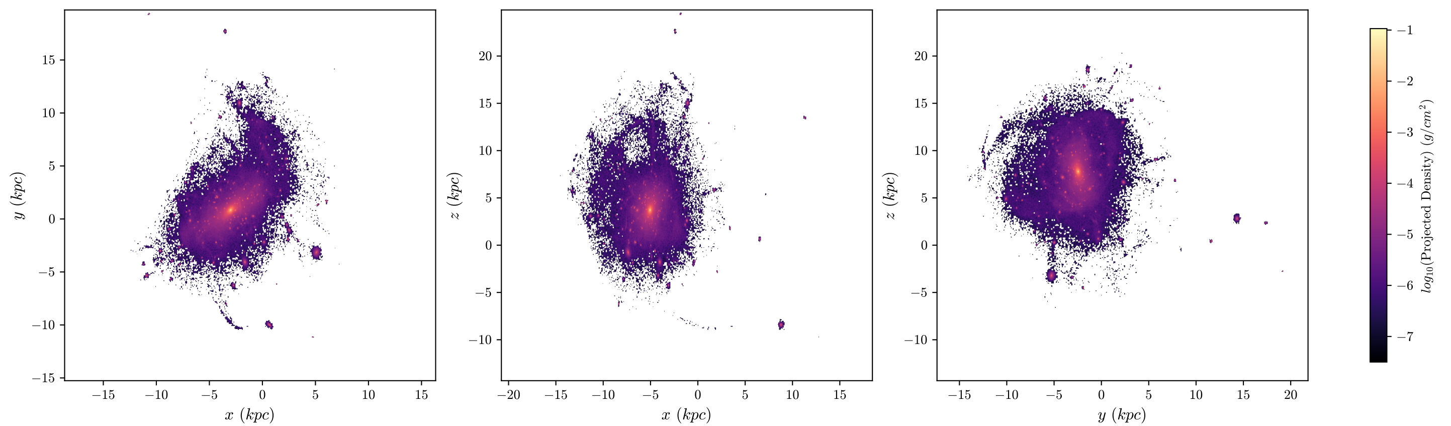
T1 Aug Stars, z = 1.313 , 512 bins
