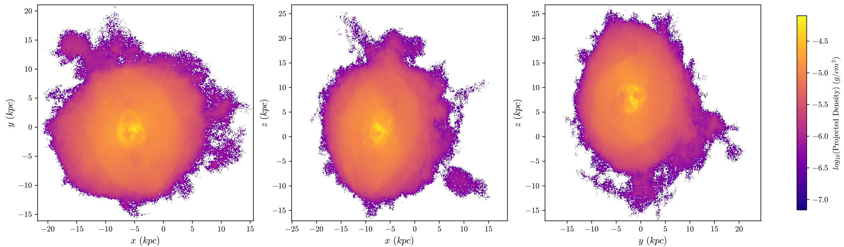
T1 Aug Dark Matter, z = 1.313 , 512 bins
