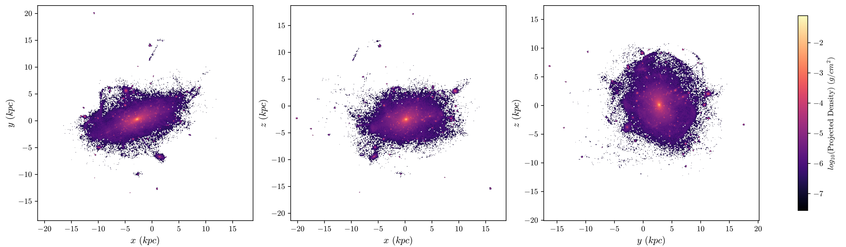
T1 Aug Stars, z = 0.997 , 512 bins
