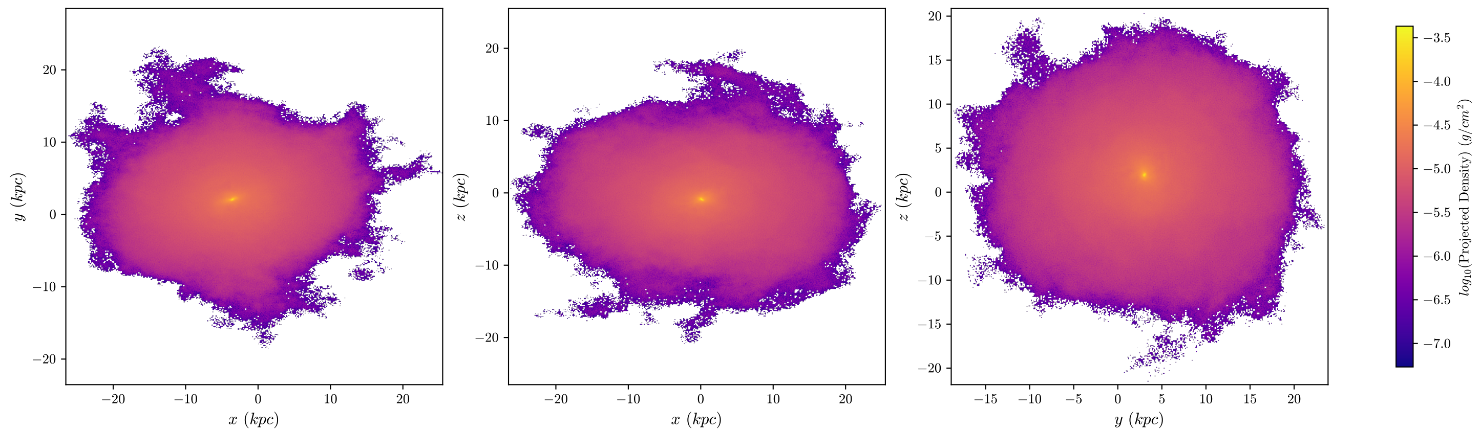
T1 Aug Dark Matter, z = 0.997 , 512 bins
