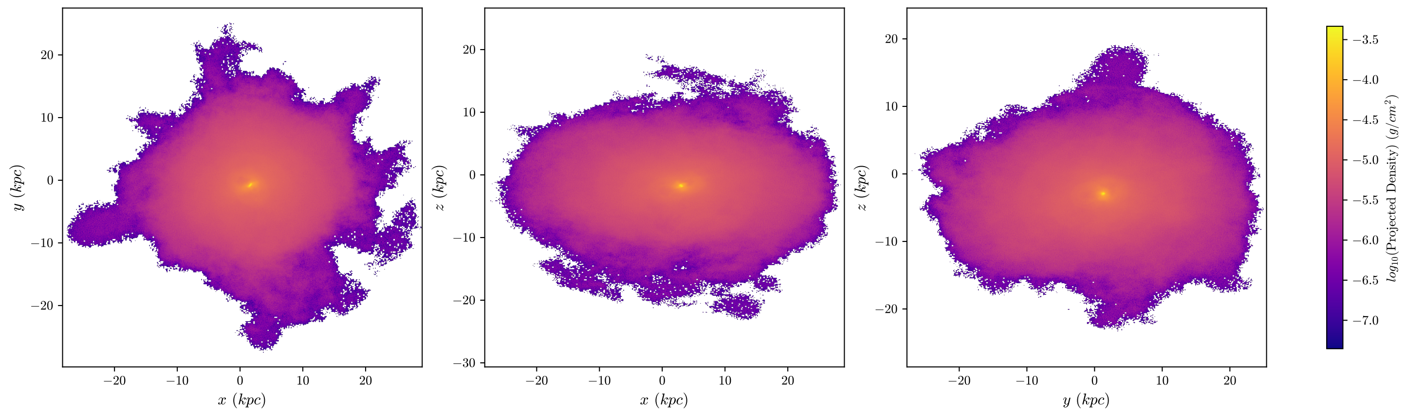
T1 Aug Dark Matter, z = 0.914 , 512 bins
