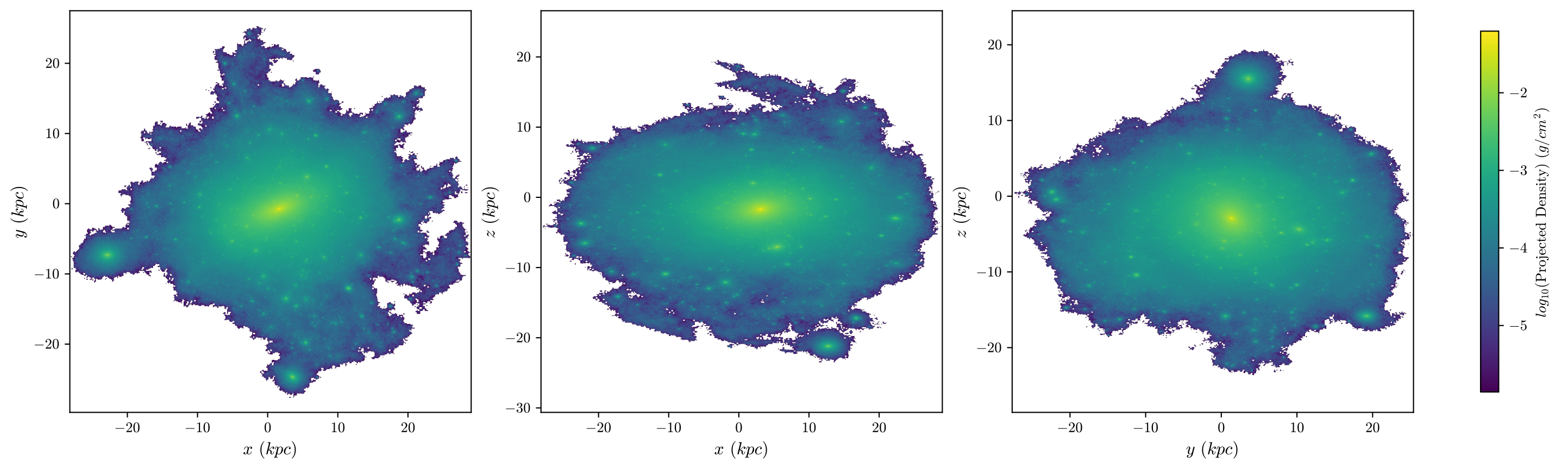
T1 Aug Stars, z = 0.914 , 512 bins
