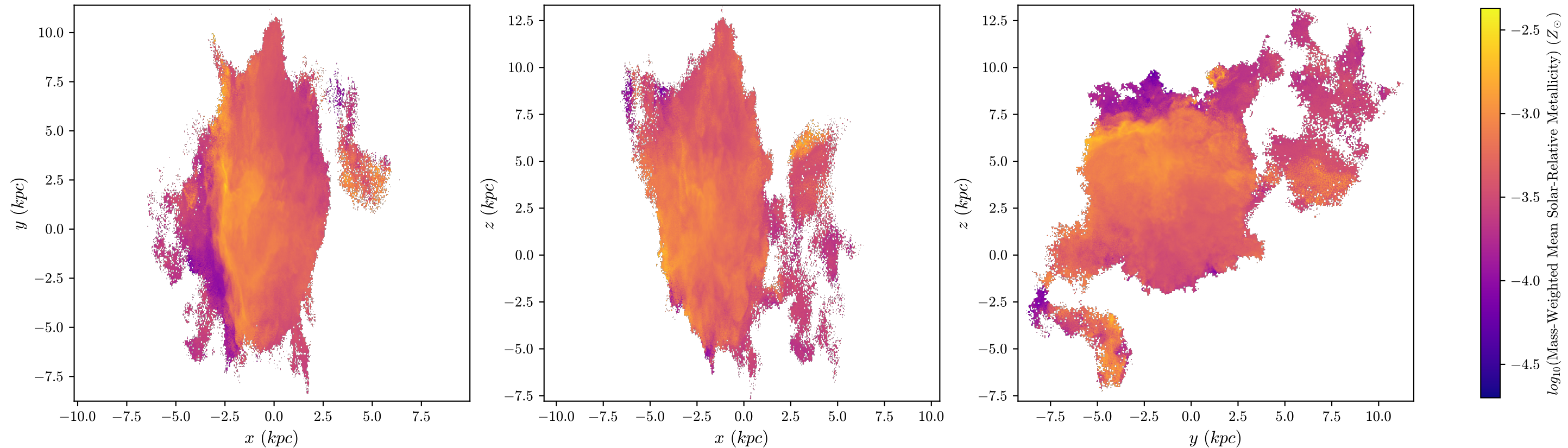
T1 Aug Mass-Weighted Mean Metallicity, z = 4.008 , 512 bins
