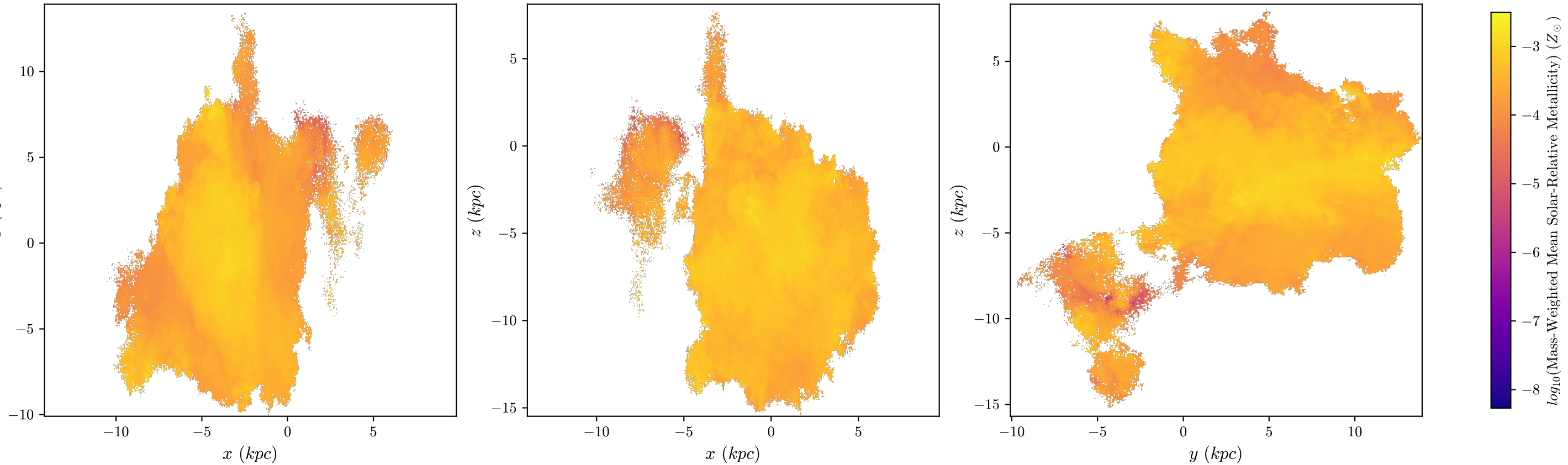
T1 Aug Mass-Weighted Mean Metallicity, z = 3.344 , 512 bins
