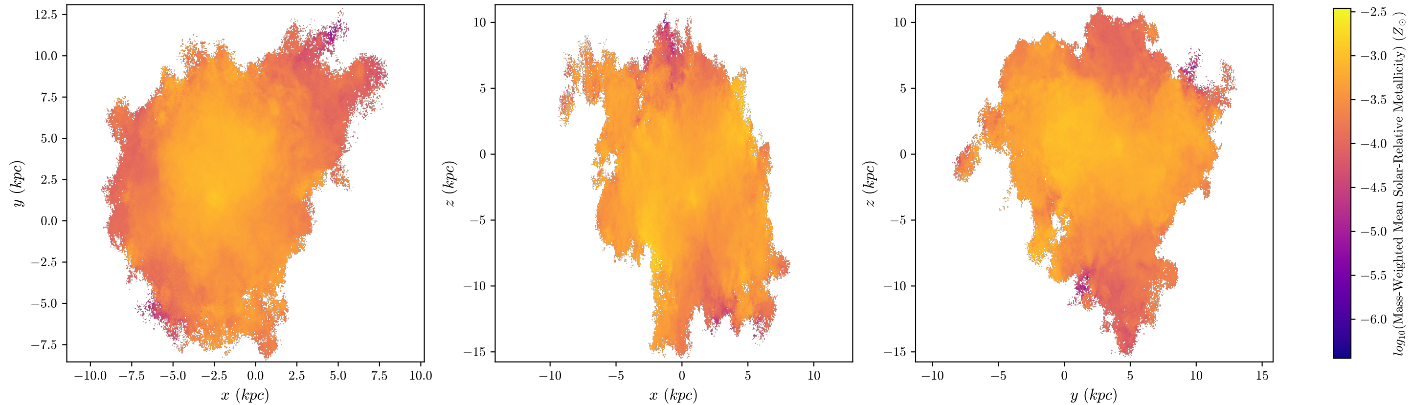
T1 Aug Mass-Weighted Mean Metallicity, z = 2.859 , 512 bins
